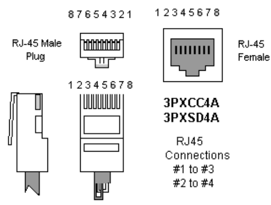
CONNECTIONS - Models With Echo Jumper
